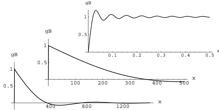
Fig.2: the CLCQ function g_B(x^-) at different spatial scales.
